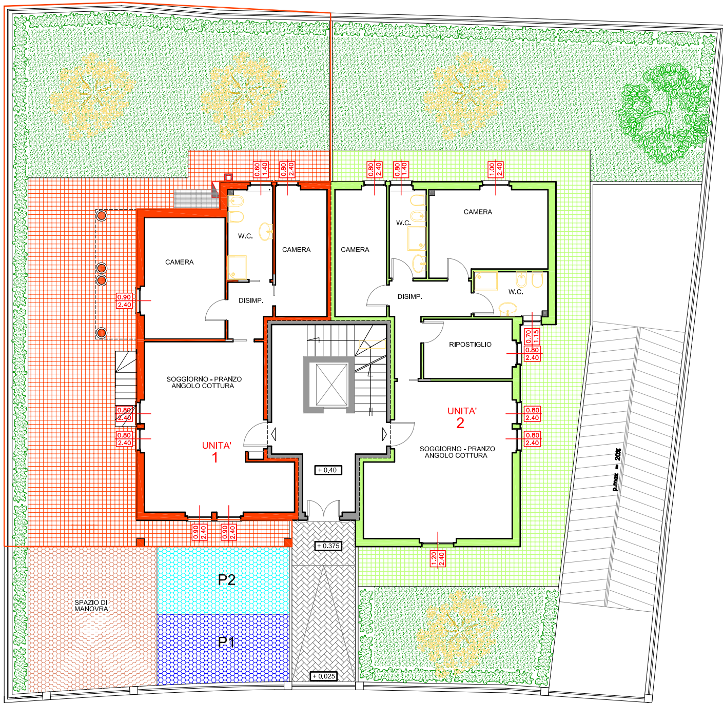
PIANO TERRA
